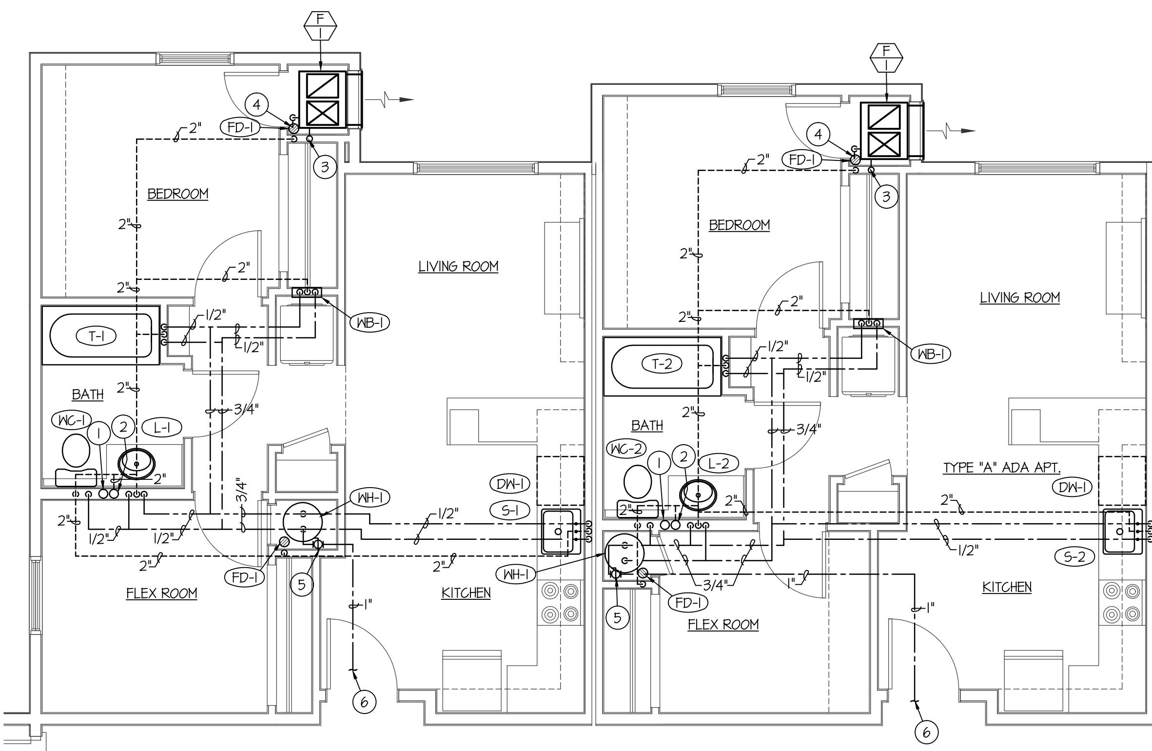
TYPICAL MAIN LEVEL APTS. WATER, GAS AND VENT PIPING FLOOR PLANS
