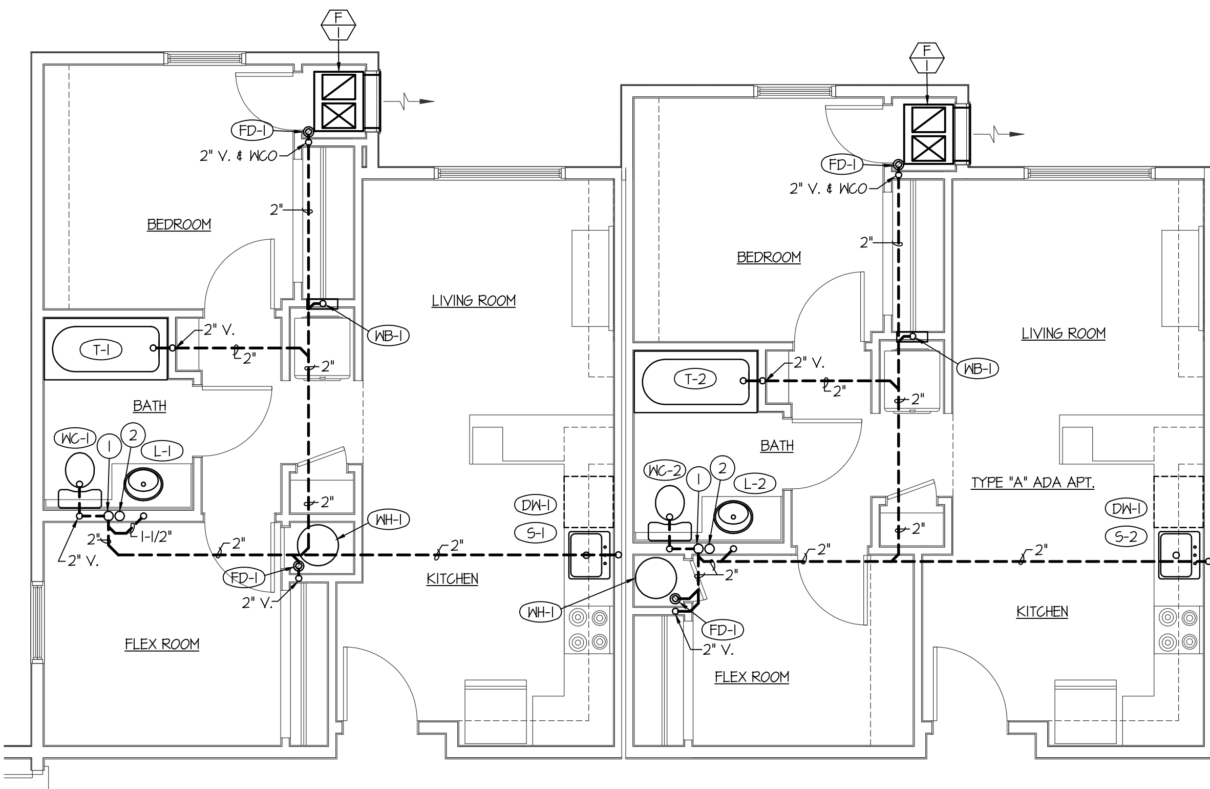
TYPICAL MAIN LEVEL APTS. WASTE PIPING FLOOR PLANS
