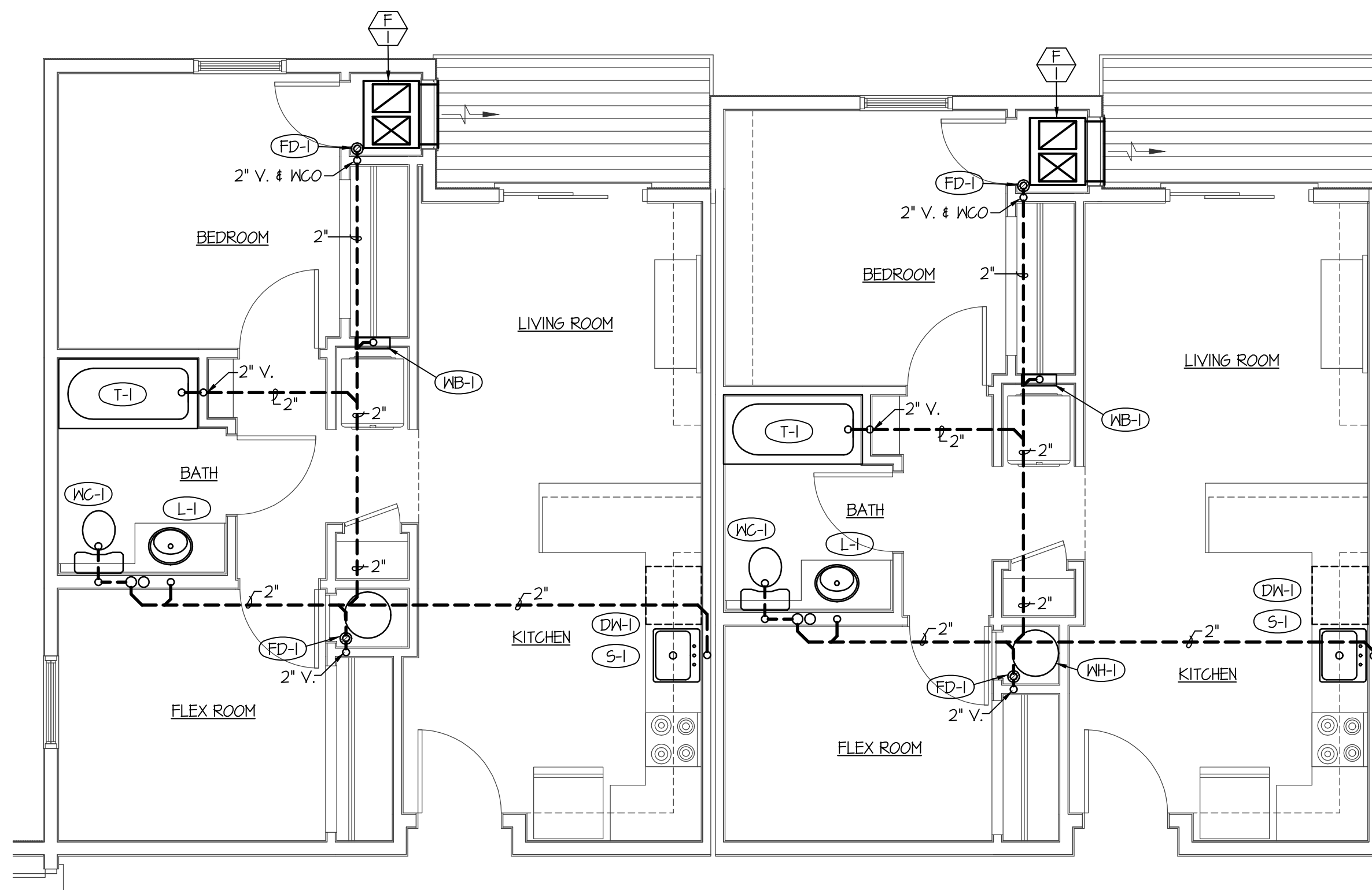
TYPICAL ONE & TWO BED RM. APTS WASTE PIPING FLOOR PLANS
