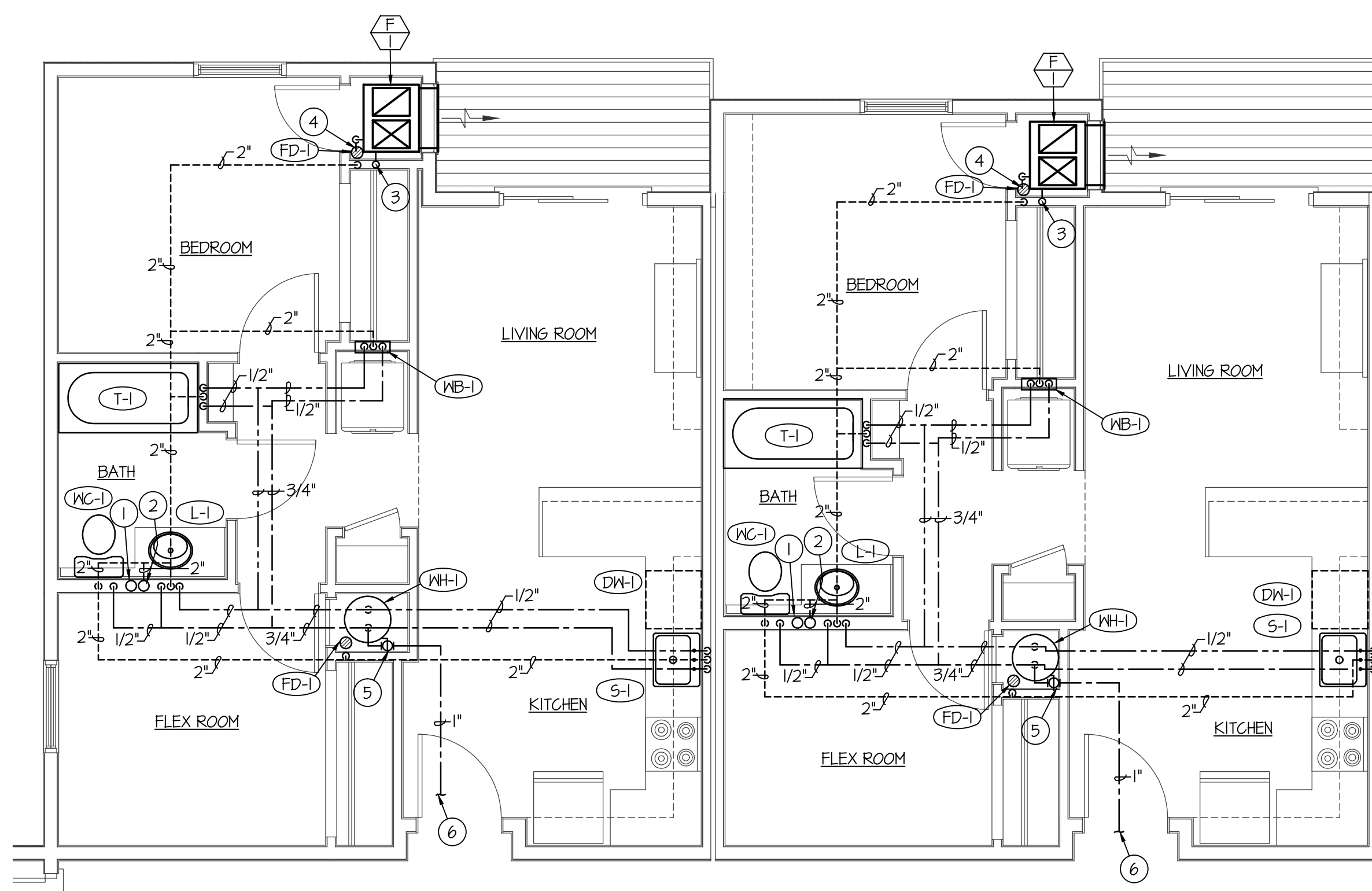
TYPICAL ONE & TWO BED RM. APTS WATER, GAS AND VENT PIPING FLOOR PLANS
